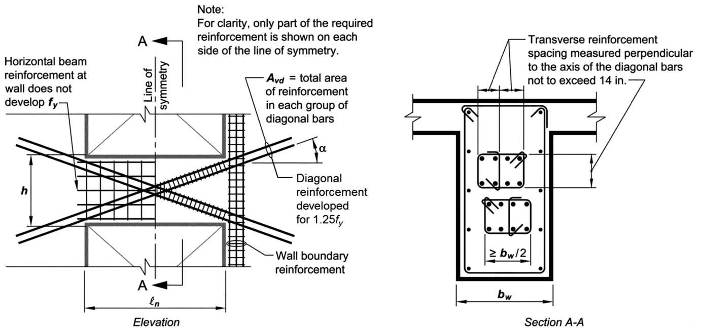
(a) Confinement of individual diagonals
