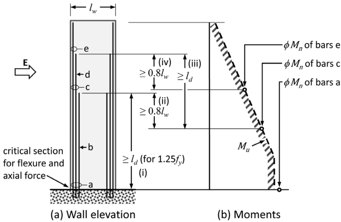
Figure 5-9 – Bar cutoffs for vertical reinforcement for idealized M_u moment diagram.
