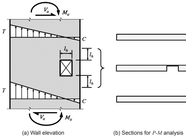
Figure 5-18 – P - M analysis at irregular opening.
