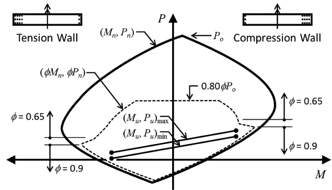
Figure 5-17 – P - M capacity check for coupled walls.
