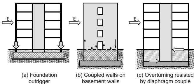
Figure 2-6 – Various ways to spread overturning resistance.
