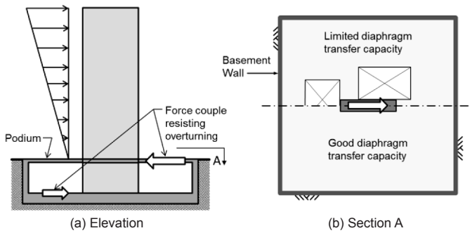
Figure 2-5 – Force transfers between walls and diaphragms.
