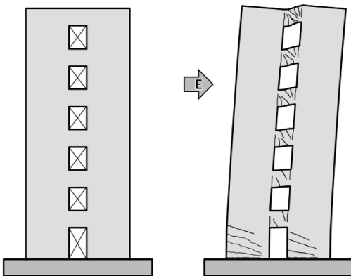
Figure 2-9 – Coupled wall geometry and target yield mechanism.
