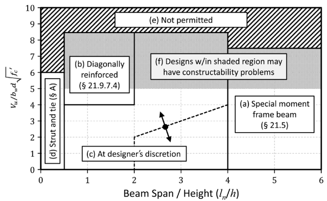
Figure 5-11 – Seismic coupling beam design space.
