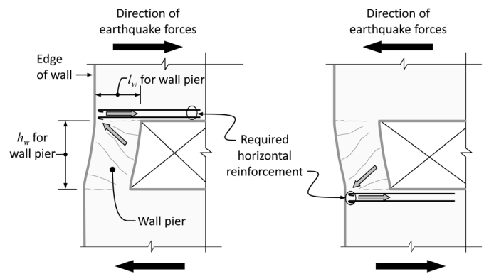
Figure 5-10 – Reinforcement required above and below wall pier.
