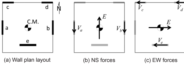
Figure 2-2 – Example plan layout. C.M. refers to center of mass.
