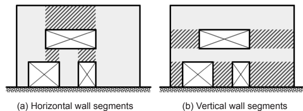
Figure 2-8 – Vertical and horizontal wall segments (hatched).
