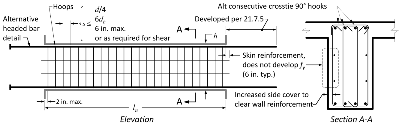
Figure 5-12 – Details for conventionally reinforced coupling beams.
