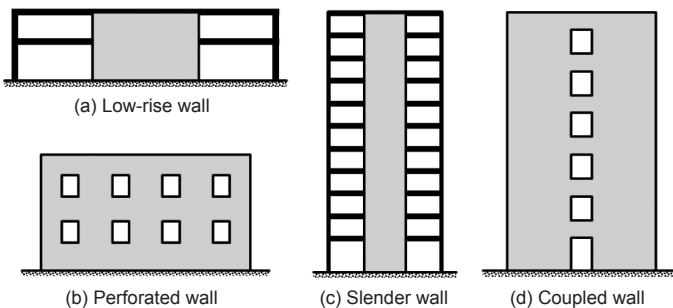
Figure 2-1 – Some illustrative structural wall elevations.
