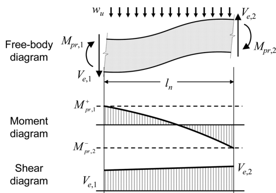
Figure 5-13 – Design shear for conventionally reinforced coupling beam. Reversed loading case also must be considered.
