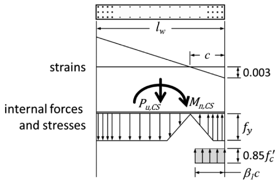
Figure 5-4 – Calculation of neutral axis depth c .
