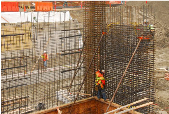
Figure 7-3 – Boundary confinement for wall flange.
