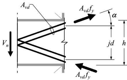
Figure 5-15 – Free-body diagram of half-span of a diagonally reinforced coupling beam. (Gravity loads not shown.)
