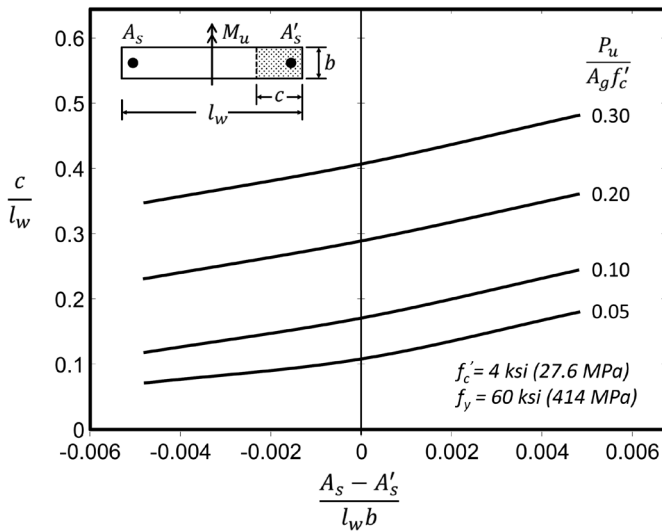
Figure 5-2 – Approximate flexural compression depth. For flanged sections, adjust A_s , A'_s , and b considering effective flange width.
