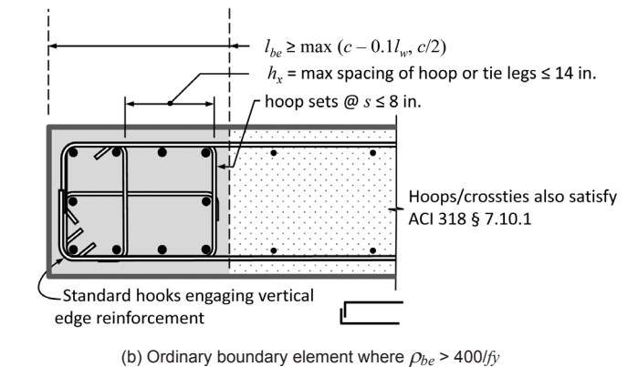
Figure 5-3 – Special and ordinary boundary elements.
