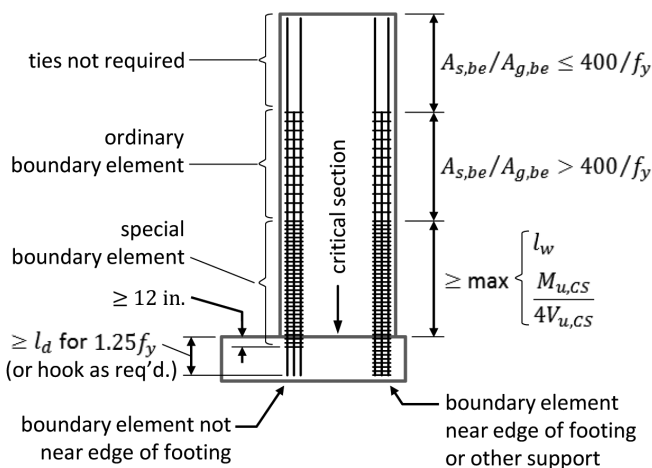
Figure 5-5 – Boundary element extensions for walls designed by Method I, for critical section at foundation interface. For ordinary and special boundary element details, see Figure 5-3 .
