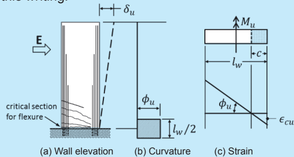
Figure 5-7 – Model to determine confinement trigger.
