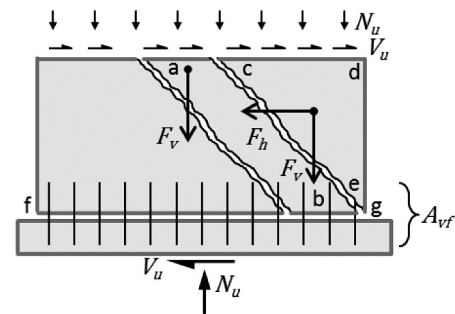
Figure 3-6 – Shear yielding and shear sliding in a squat wall.
