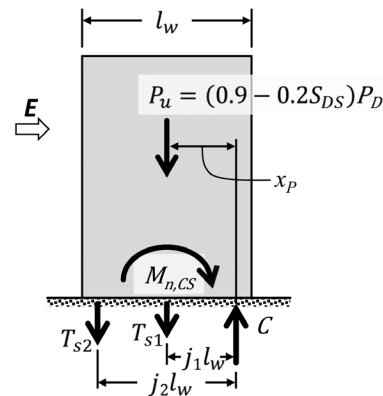
Figure 5-1 – Model for initial selection of flexural tension reinforcement.
