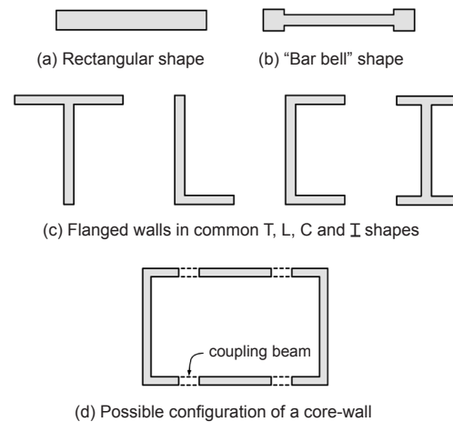
Figure 2-7 – Various wall cross sections.
