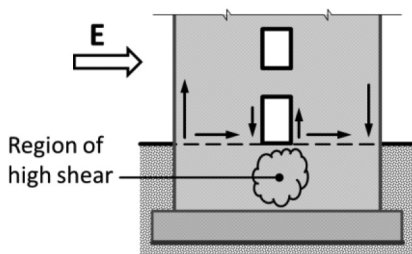
Figure 5-19 – Forces in solid wall below or above row of openings.
