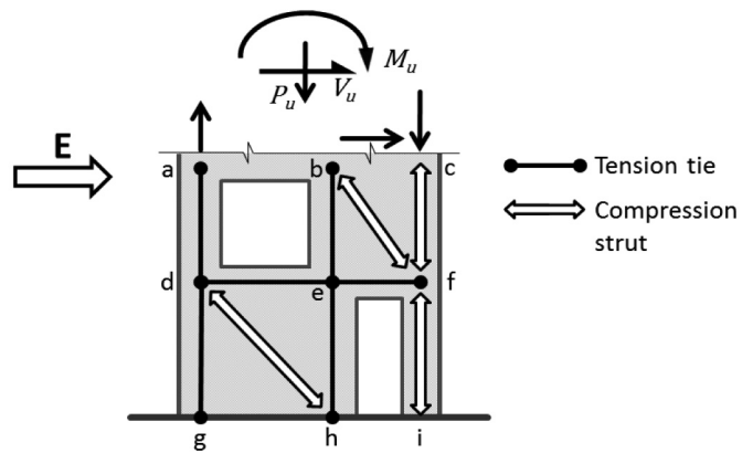
Figure 5-20– Strut-and-tie model.
