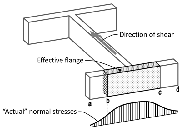
Figure 4-1 – Effective flange activation.
