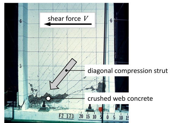
Figure 3-4 – Web crushing due to high shear force in laboratory test.
