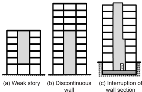
Figure 2-3 – Wall vertical irregularities.
