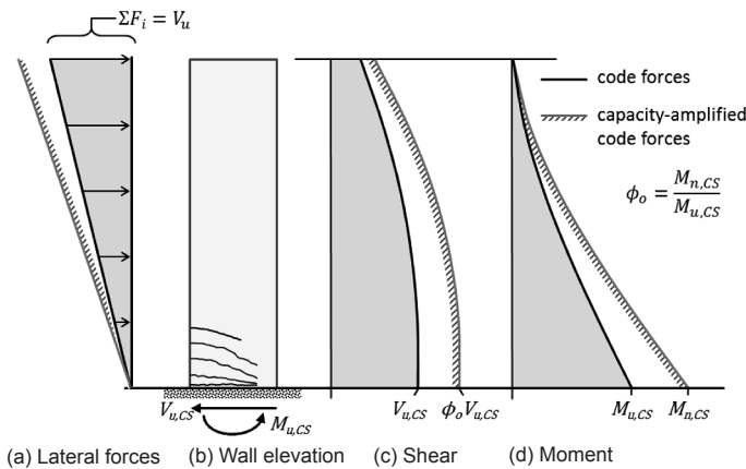
Figure 3-5 – Wall lateral forces, shears, and moments; code-prescribed forces and code-prescribed forces corresponding to development of nominal flexural strength.
