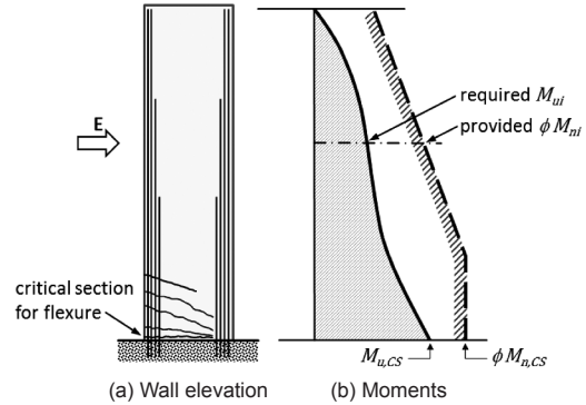
Figure 3-1 – Provided versus required flexural strength in a wall with a single critical section.
