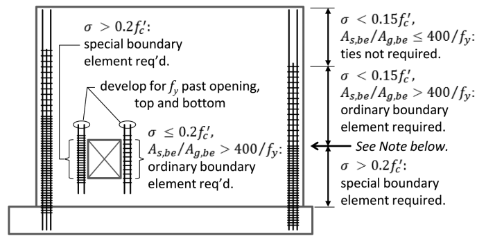
Note: Requirement for special boundary element is triggered if \sigma > 0.2f'_c . Once triggered, the special boundary element extends until \sigma < 0.15f'_c .
