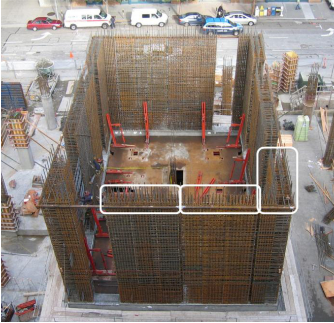
Figure 7-1 – Pre-tied modules (some modules encircled).
