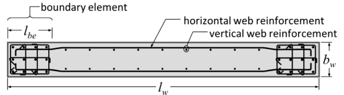
Figure 2-10 – Typical reinforcement for rectangular wall.
