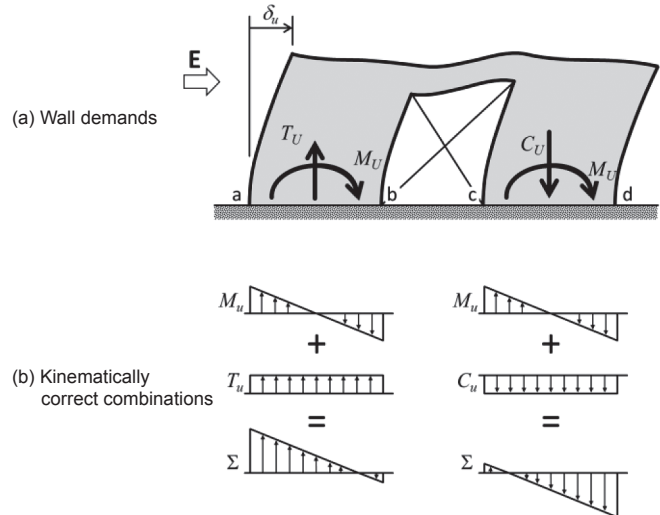
Figure 5-8 – Elevation of laterally displaced coupled wall system.
