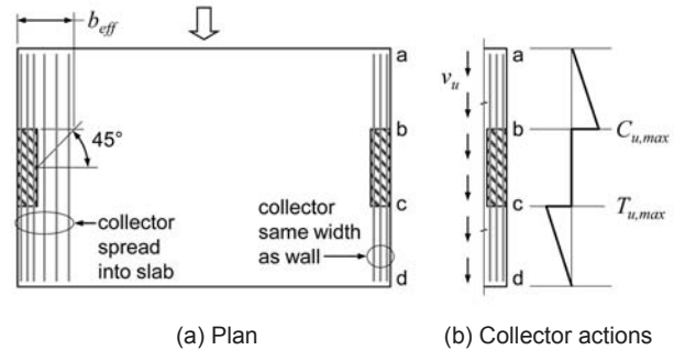
Figure 3-2 – Collectors.
