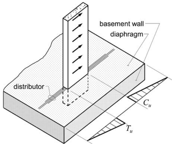
Figure 3-3 – Distributor.
